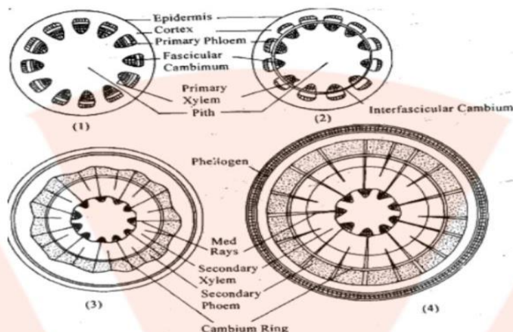
Fig: Diagram showing secondary growth in Dicot Stems
