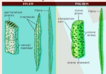
Fig. : Complex tissues – Xylem and phloem.
