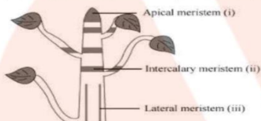
Fig : Diagram showing different types of meristems.
